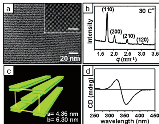
Figure 2. (a) TEM images of ultramicrotomed films 1 stained with RuO 4 revealing columnar array of alternating light-colored PEO layers and dark aromatic layers. (Inset) Image at perpendicular beam incidence; a 2-D body-centered rectangular ordered array of aromatic core (Scale bar: 10 nm). (b) Small-angle X-ray diffraction pattern of 1 measured at 30 °C. (c) Schematic representation for the formation of the 2-D body-centered rectangular columnar structure of 1 . (d) CD spectrum of 1 in aqueous solution (0.005 wt %) at 25 °C.
